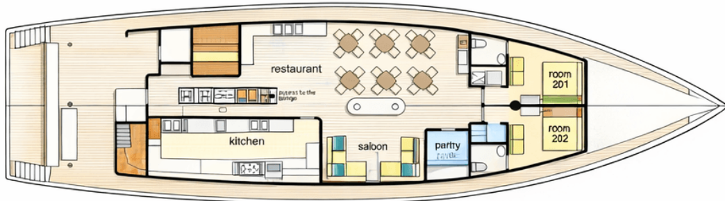
ari queen main deck main deck LWL 107ft4" (32m74) Width 32m1 - 9m84
