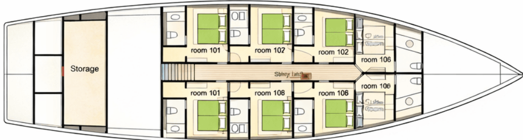
ari queen lower deck Lower deck LWL 107ft4" (32m74) Width 32m1 - 9m84
